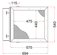
End View Air Inlet
