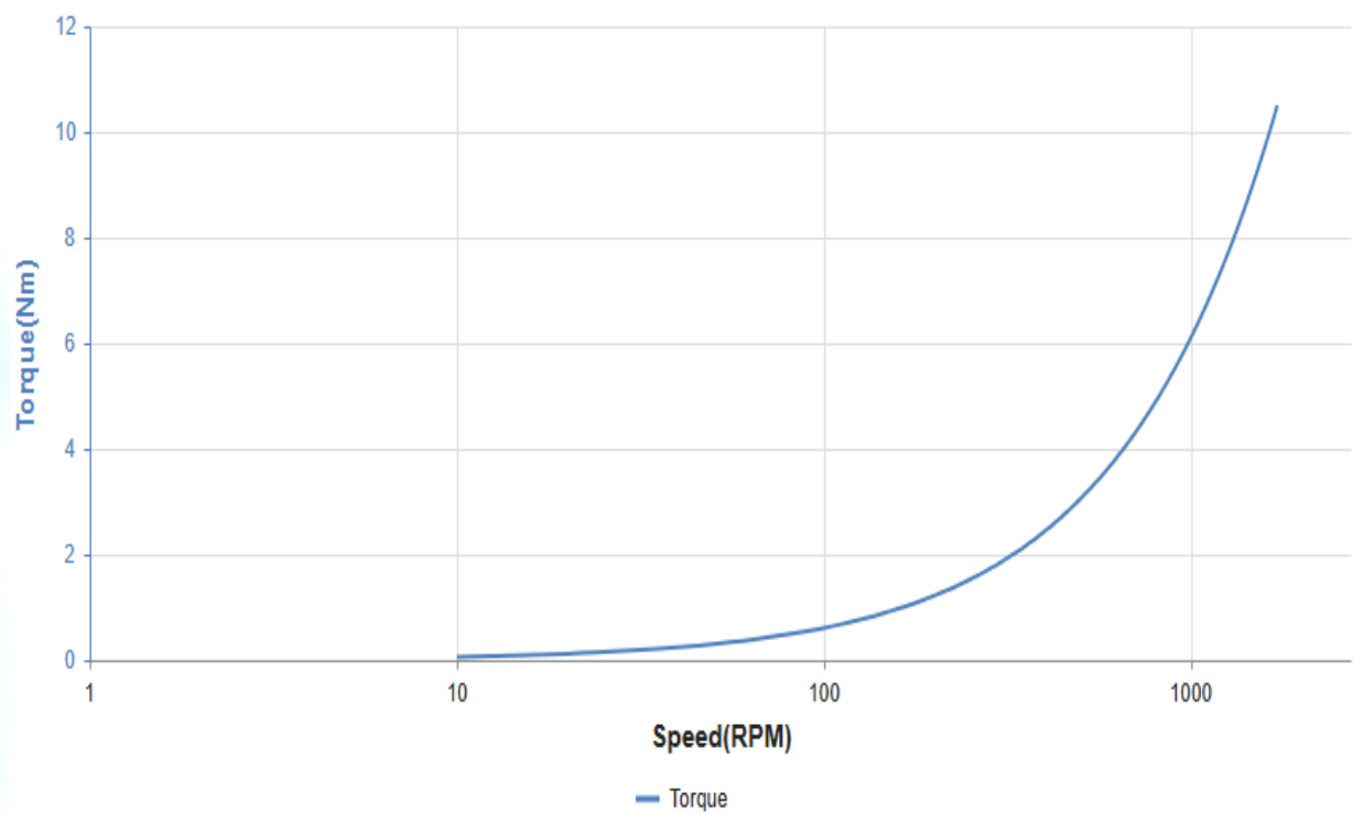
Speed Torque Curve
