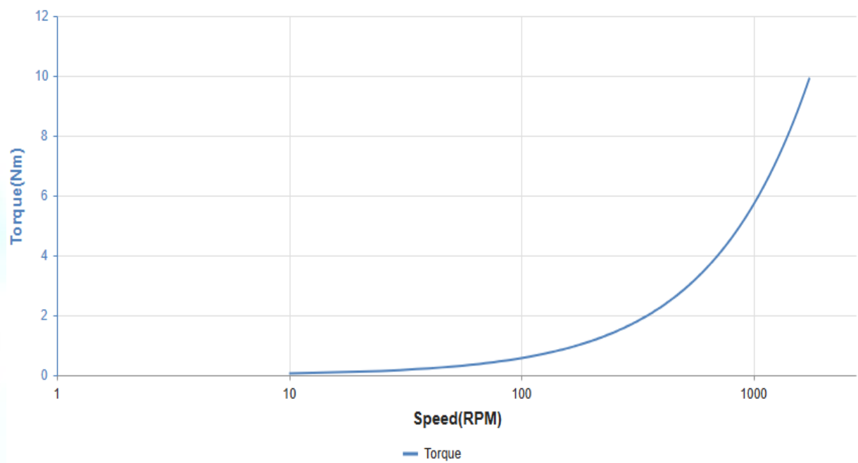
Speed Torque Curve
