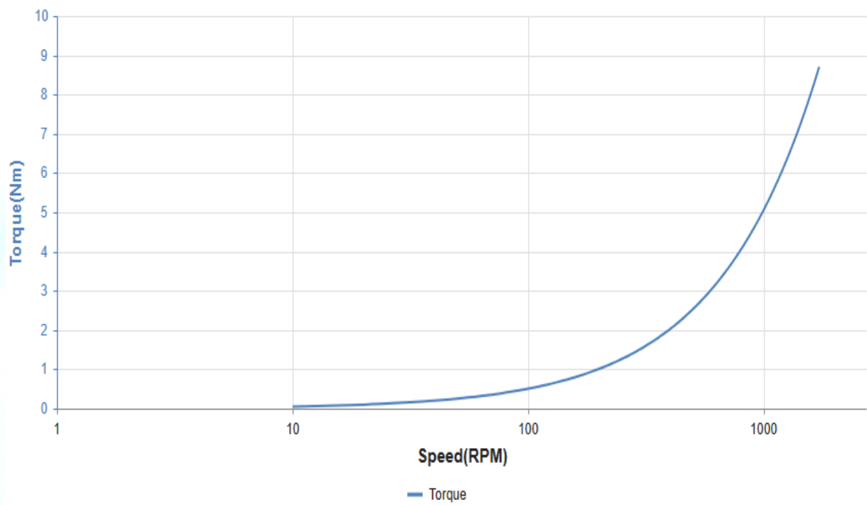
Speed Torque Curve
